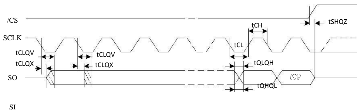
Figure 37. Output Timing
